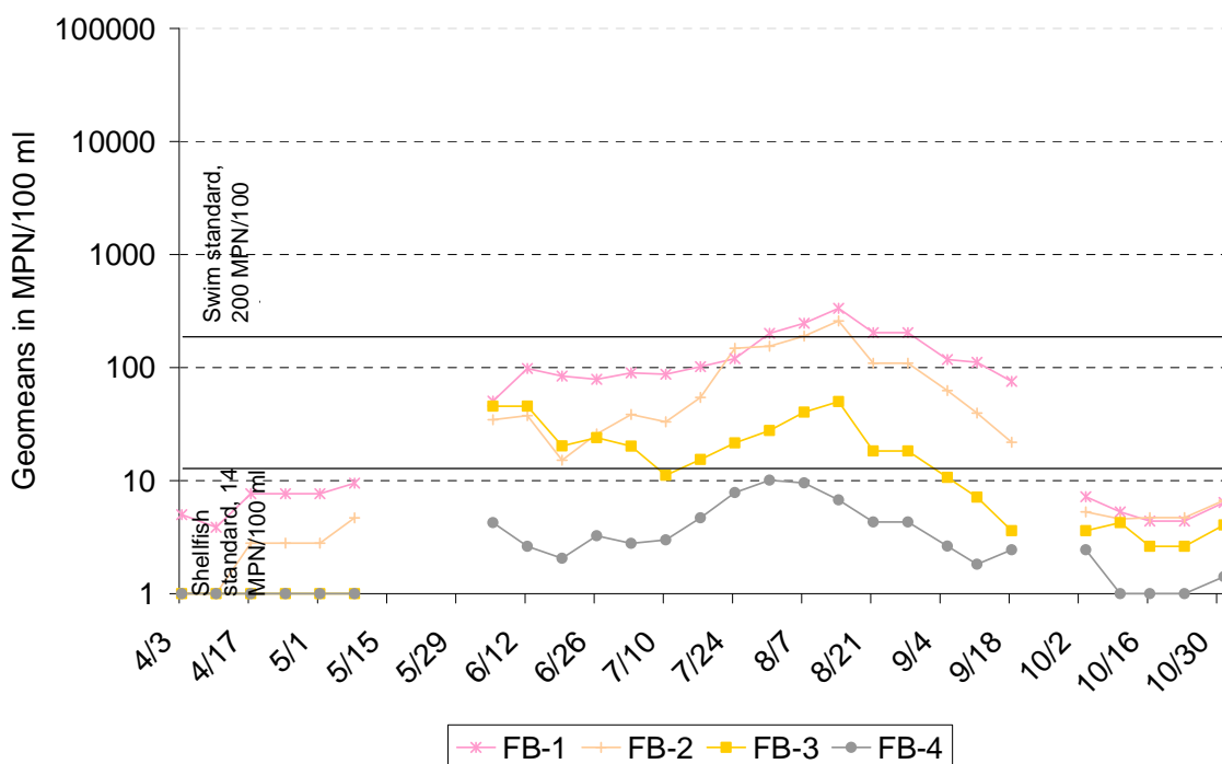
Figure 6. 30-day running geometric mean of 2006 Cold Spring Harbor fecal coliform samples
